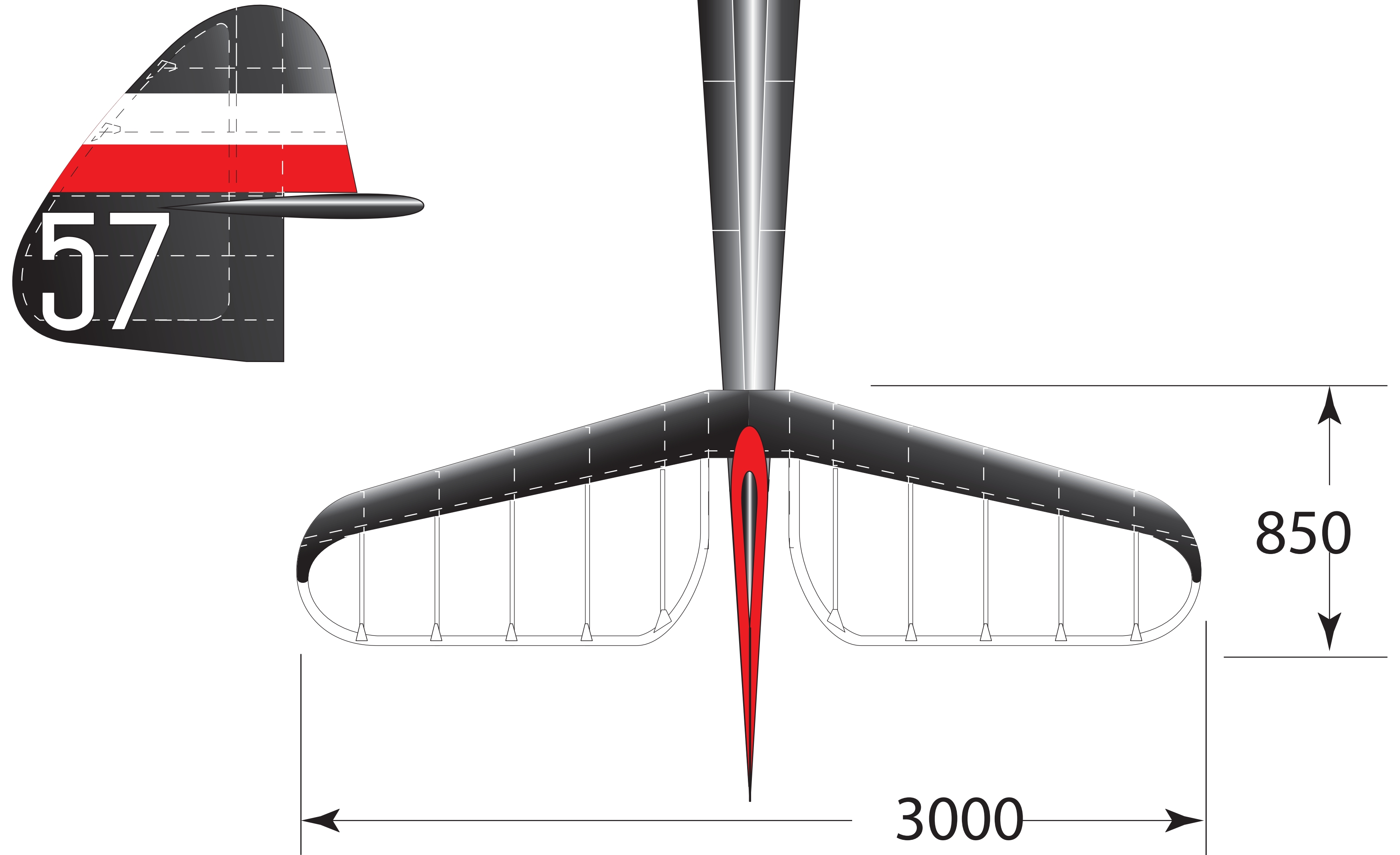
Minimoa Prototype - built in 1935 by Schempp-Hirth Segelflugzeugbau
